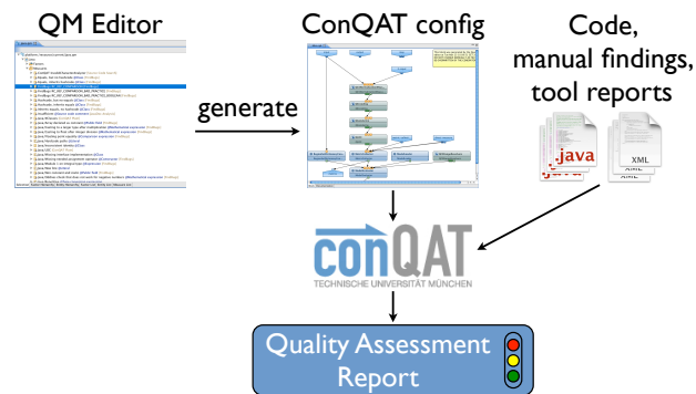
Figure 1: Quamoco Tool Chain
