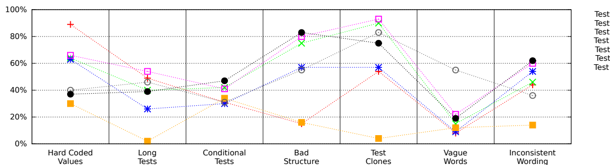
Fig. 2. Percentage of Tests Affected by Smells.
